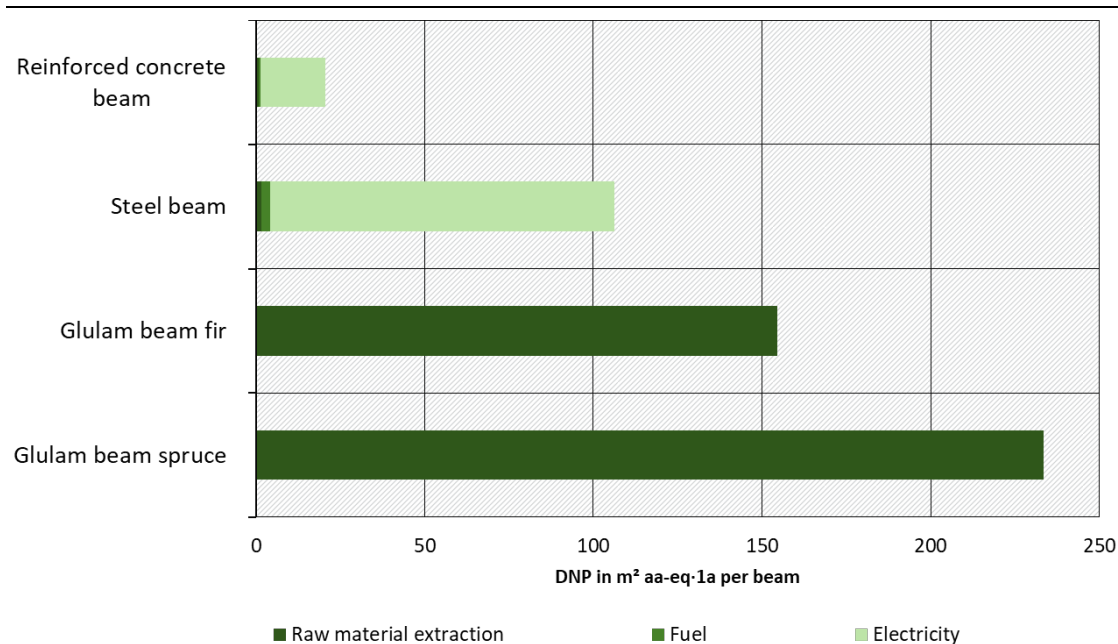
Figure 5: Distance-to-nature potential (DNP) for temporary land occupation by the analysed different hall beams
